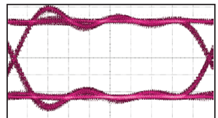
Real Time Oscilloscope
